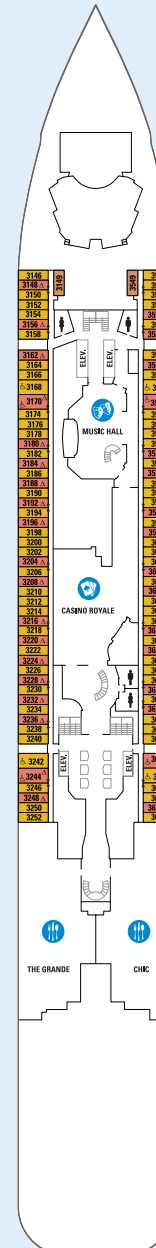
DECK 3
