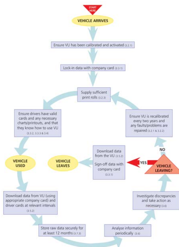
Diagram showing digital tachograph vehicle use cycle
